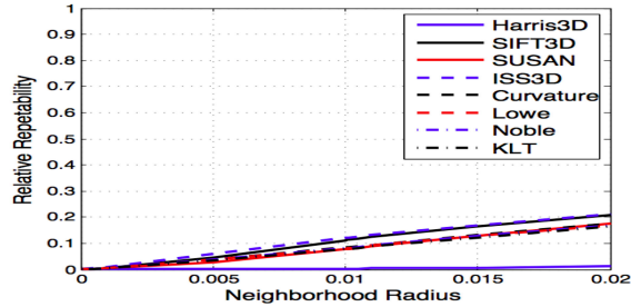
(i) Relative repeatability for 45^\circ rotation.
