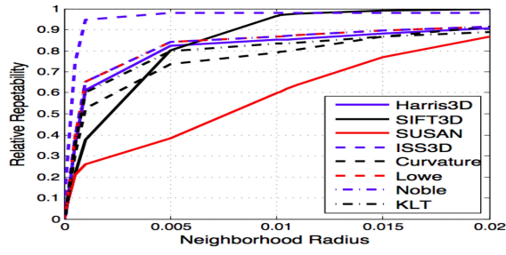
(a) Relative repeatability for 5^\circ rotation.
