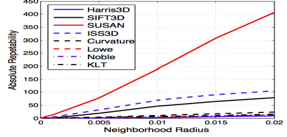
(f) Absolute repeatability for 25^\circ rotation.
