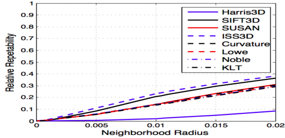
(g) Relative repeatability for 35^\circ rotation.
