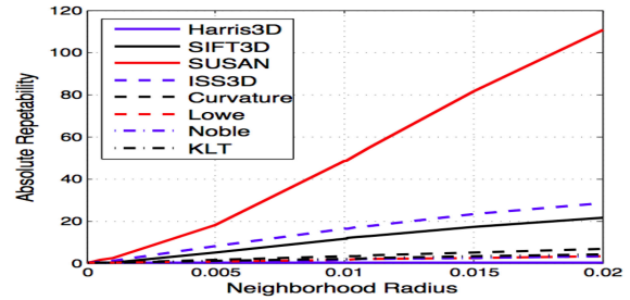
(j) Absolute repeatability for 45^\circ rotation.
