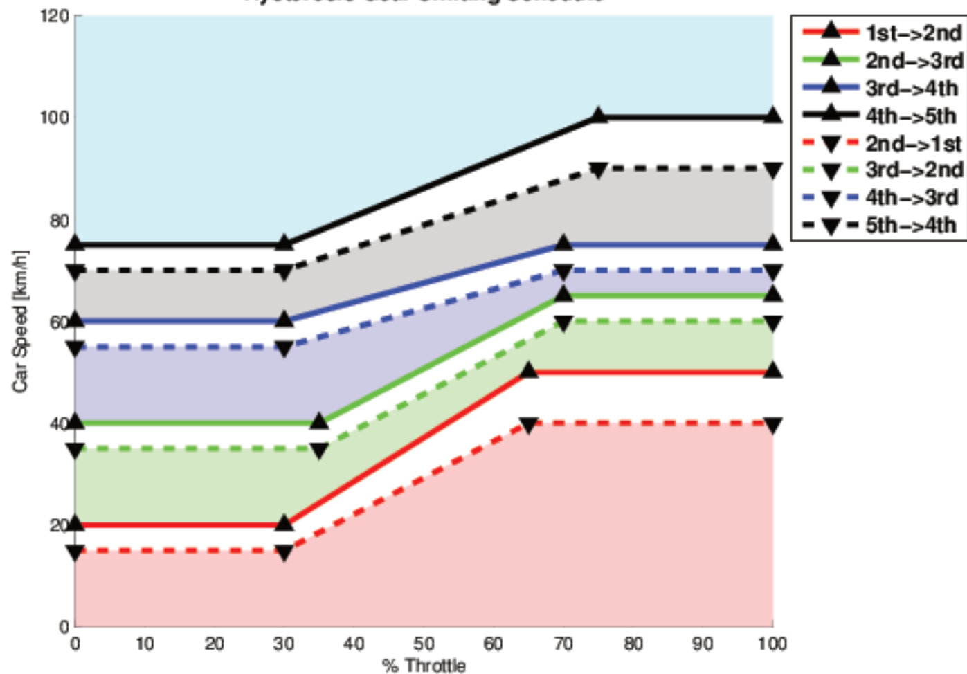
Hysteresis Gear Shifting Schedule
