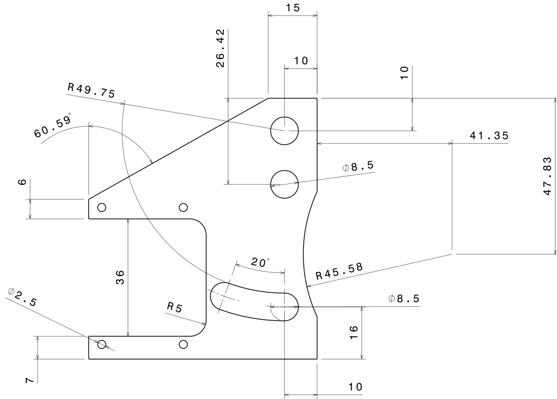
Front view Scale: 3:2
