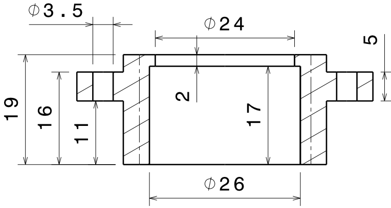
Section view B-B Scale: 3:2
