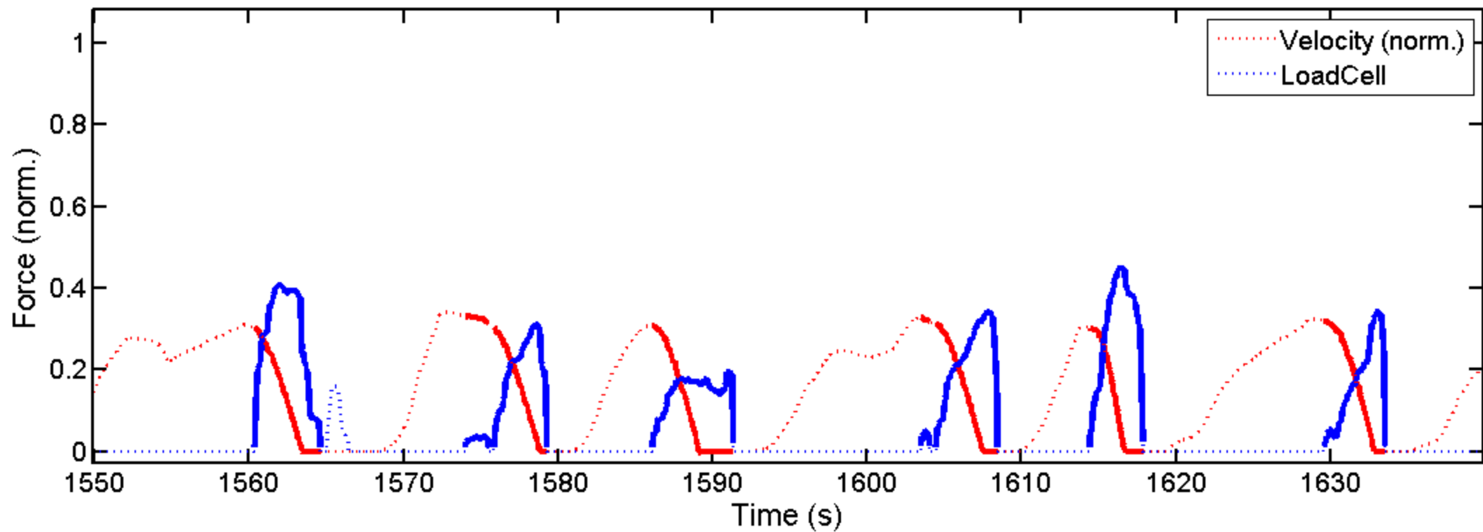
Braking test 20-0 km/h: Time vs Velocity & Forces
