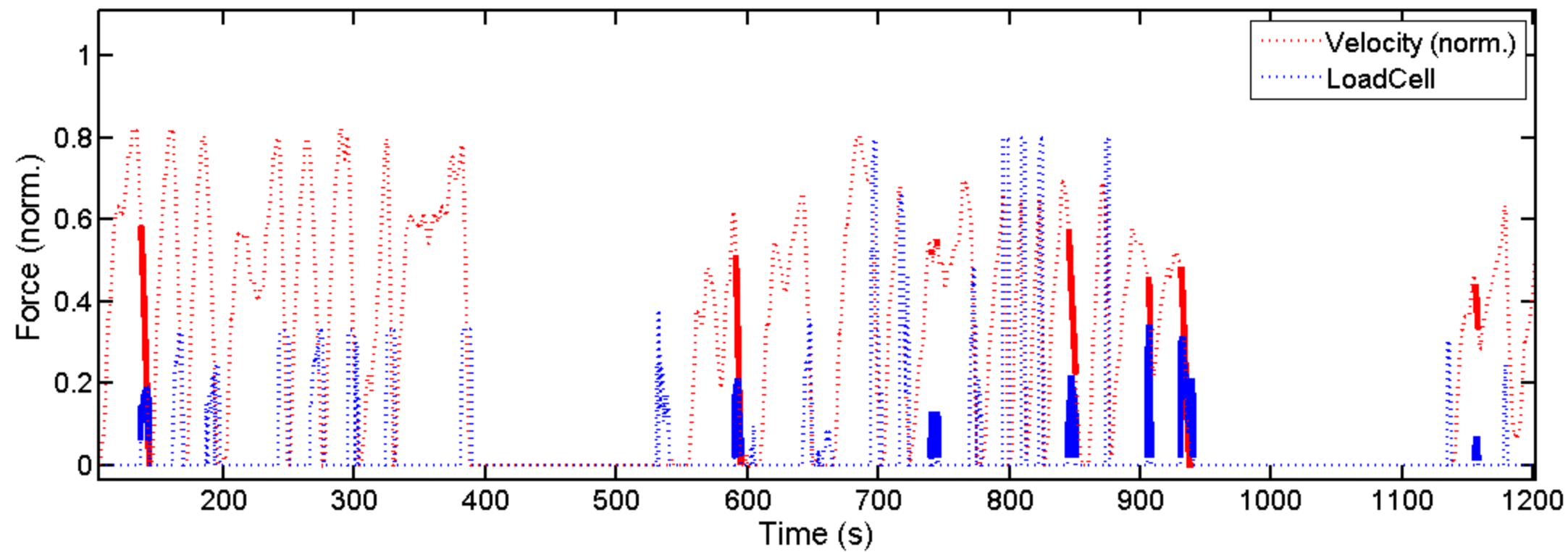
Braking test 30-0 km/h: Time vs Velocity & Forces
