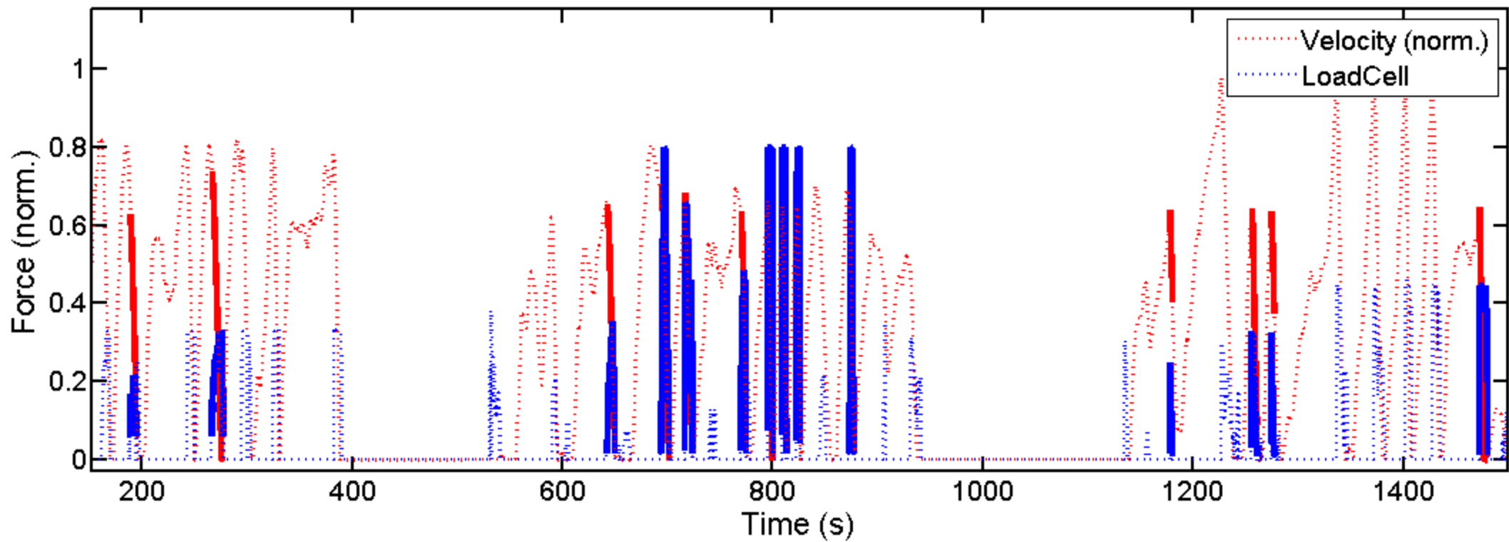
Braking test 40-0 km/h: Time vs Velocity & Forces
