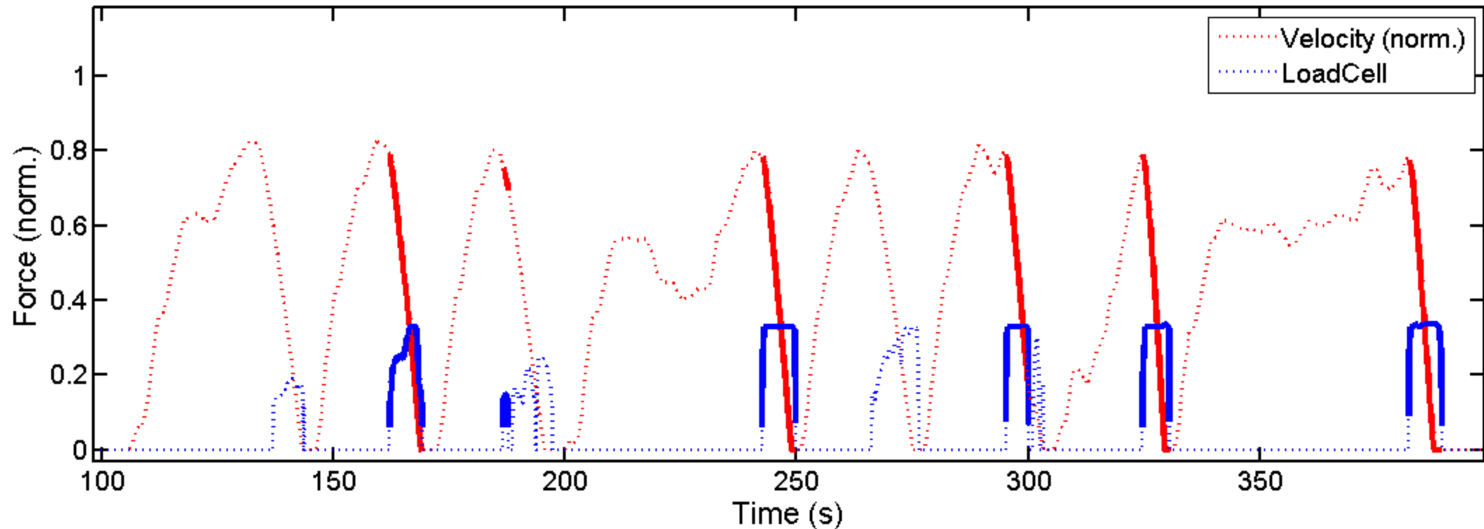
Braking test 50-0 km/h: Time vs Velocity & Forces
