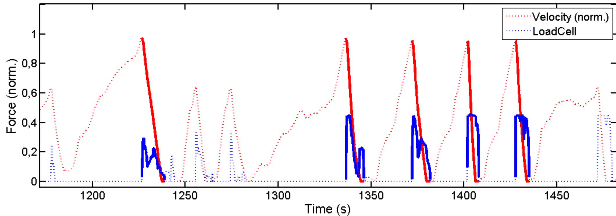
Braking test 60-0 km/h: Time vs Velocity & Forces
