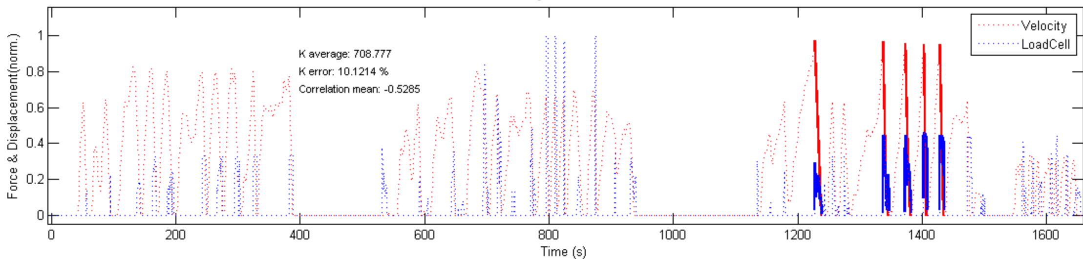
Braking test:50-0 km/h
