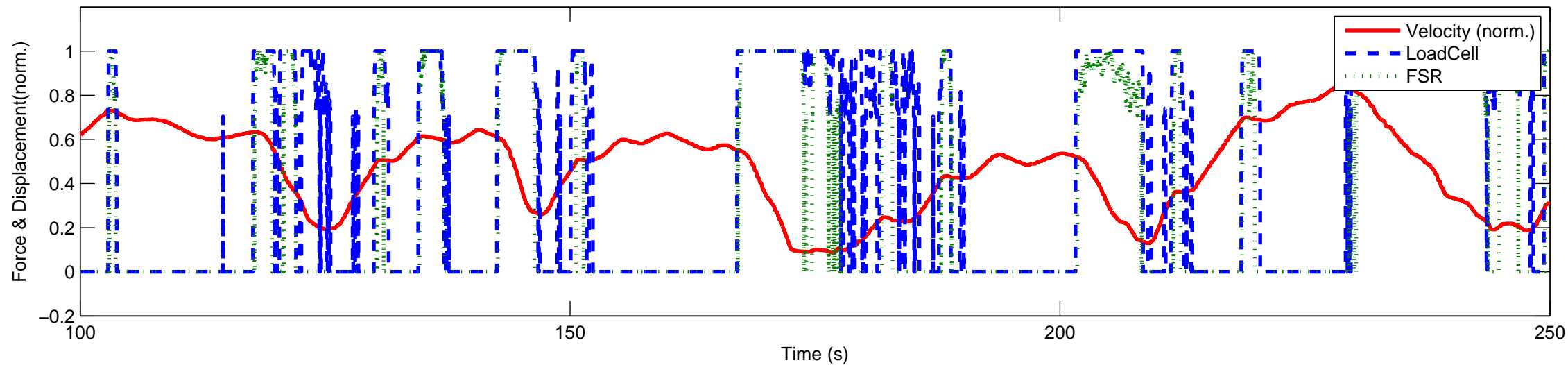
Clutch – Time vs Velocity & Forces/Displacement
