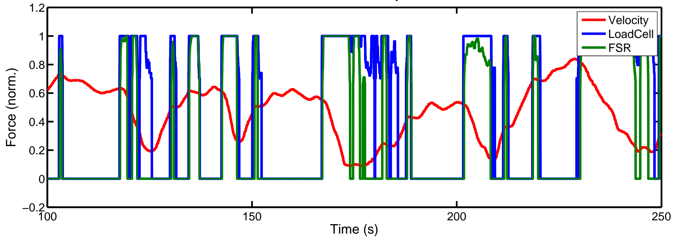
Clutch – Time vs Velocity & Forces
