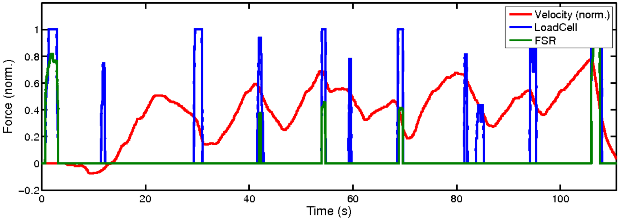
Brake – Time vs Velocity & Forces
