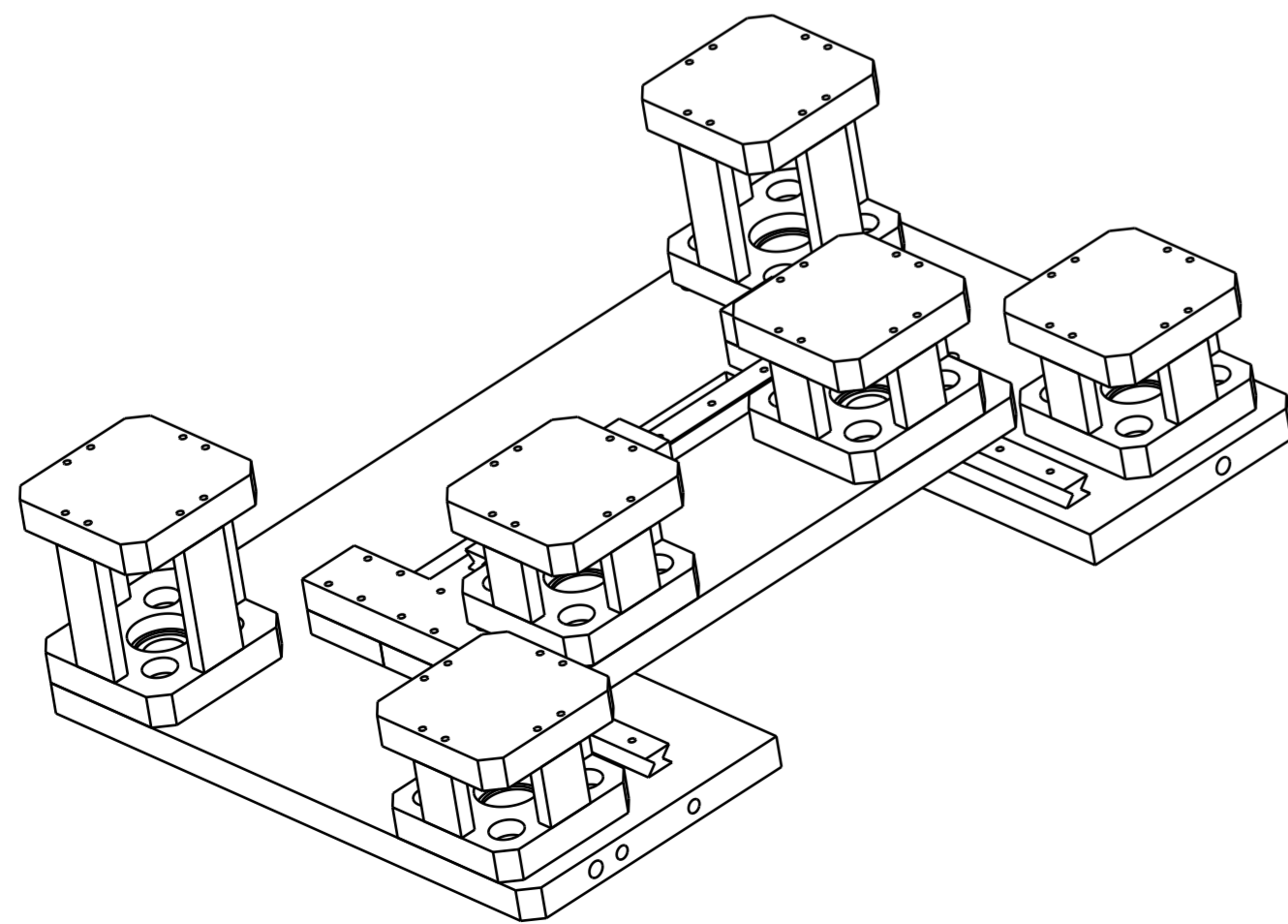
Isometric view Scale: 1:2
