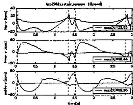
(b) Angular Velocity of Pitch Axis
