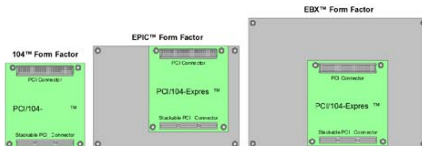
Figura 3.3: norma PC/104 vs. EBX e EPIC
