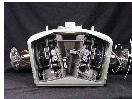
Figure 13: Chest mechanism
