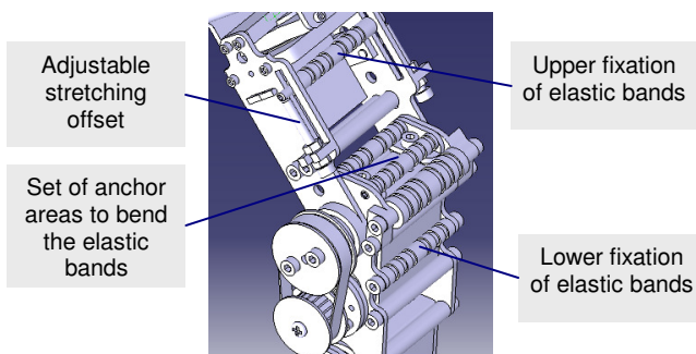
Fig. 7 - Detail of fixation and anchor points for the elastic bands.
