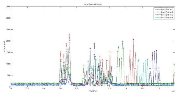
Fig. 13 – Temporal evolution of the force sensors when acting manually on the foot extremities
