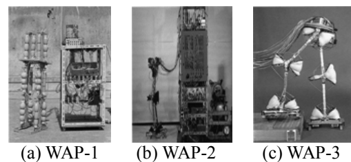
Fig. 3 WAP bipedal family developed by Professor Kato's robotic team of Waseda University in Japan where artificial muscles were introduced. WAP-1 invented in 1969, WAP-2 in 1970 and WAP-3 brought out in 1971.
