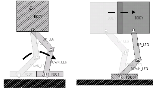
Fig. 5. Sagittal plane simulation experiments of one step leg transfer (3) and body translation (4).
