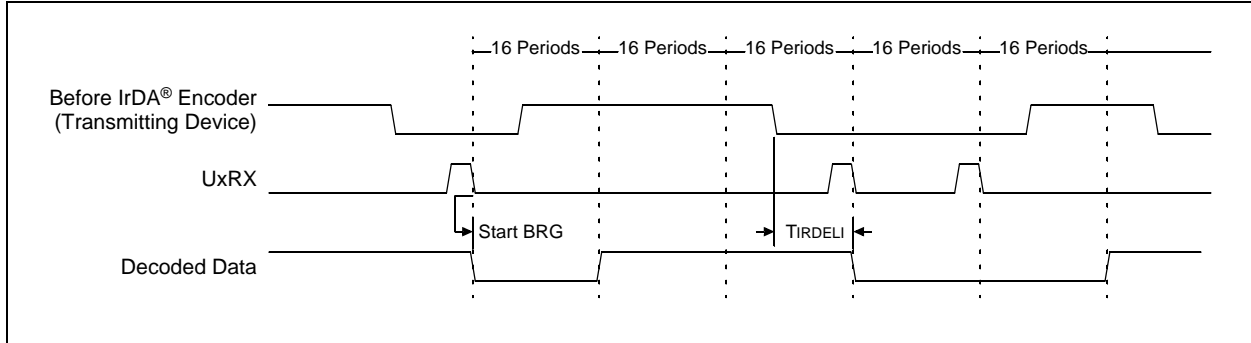
Figure 17-23: Inverted Polarity Decoding Results
