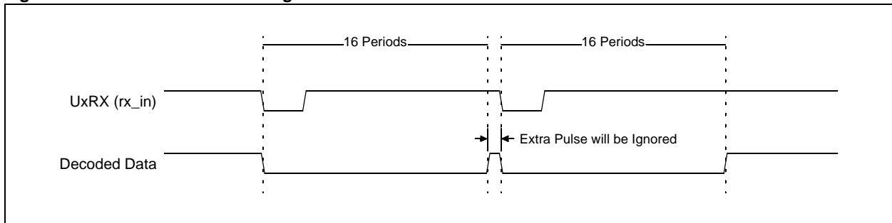
Figure 17-24: Clock Jitter Causing a Pulse Between Consecutive Zeros
