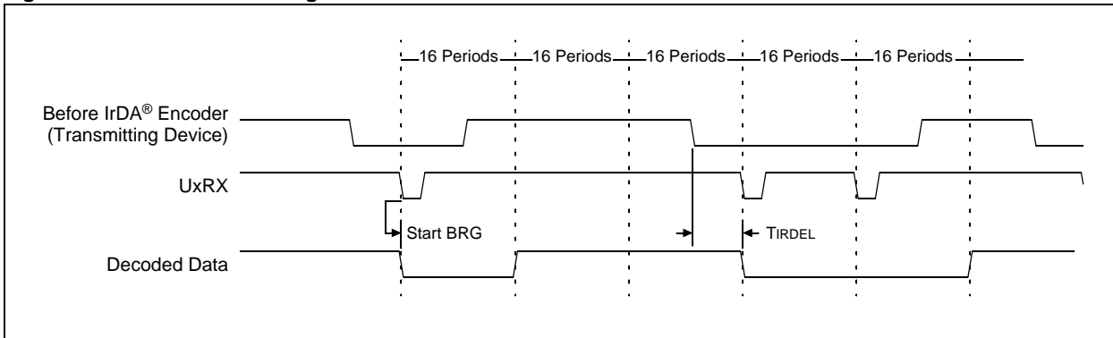
Figure 17-22: IrDA® Decoding Scheme
