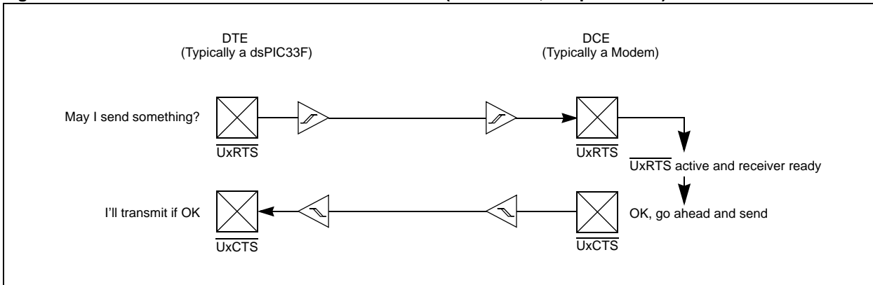
Figure 17-17: \overline{UxRTS}/\overline{UxCTS} Handshake for DTE-DCE (RTSMD = 1, Simplex Mode)
