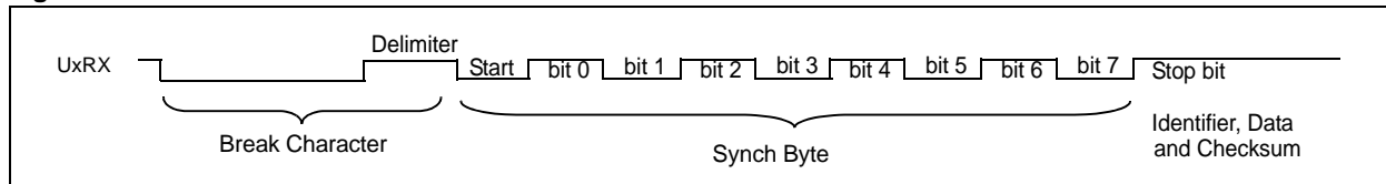
Figure 17-25: Frame Structure
