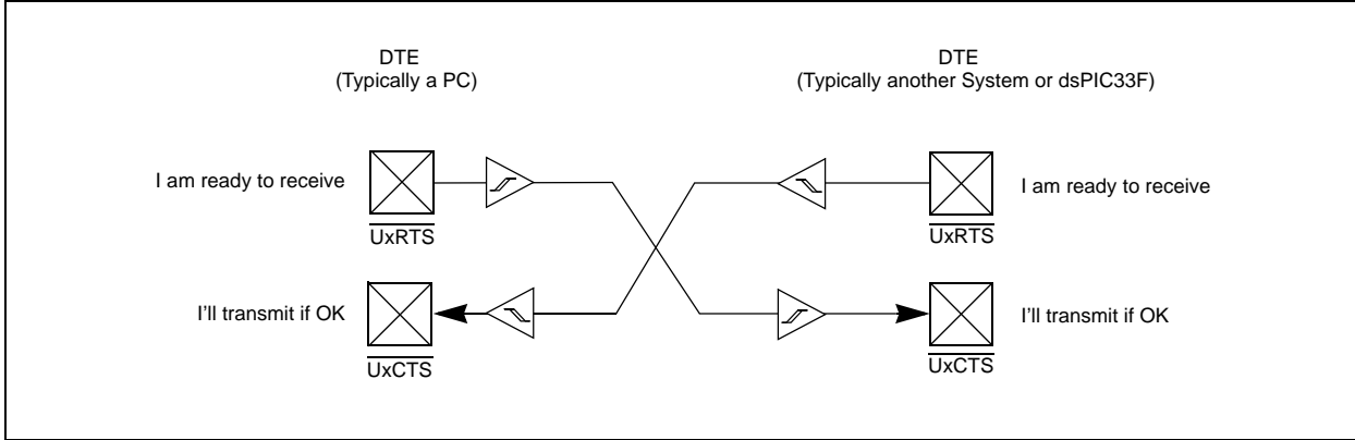
Figure 17-16: \overline{UxRTS}/\overline{UxCTS} Flow Control for DTE-DTE (RTSMD = 0, Flow Control Mode)
