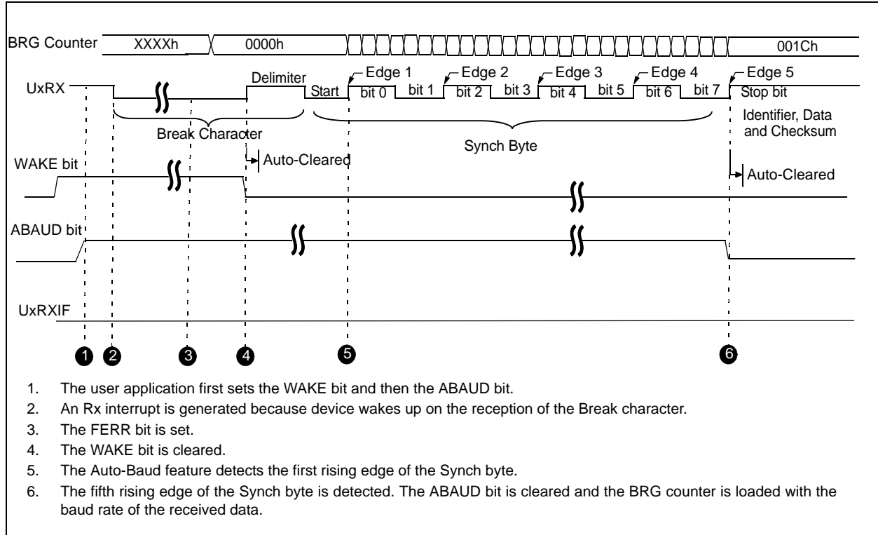
Figure 17-26: Data Reception Using the LIN Protocol
