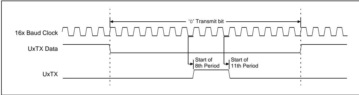
Figure 17-21: IrDA® Encode Scheme for '0' Bit Data with Respect to 16x Baud Clock
