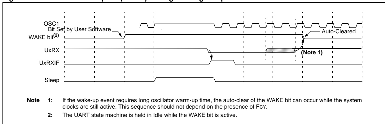
Figure 17-15: Auto-Wake-up Bit (WAKE) Timings During Sleep
