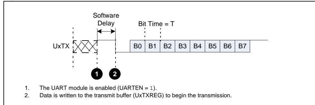
Figure 17-4: UART Transmission
