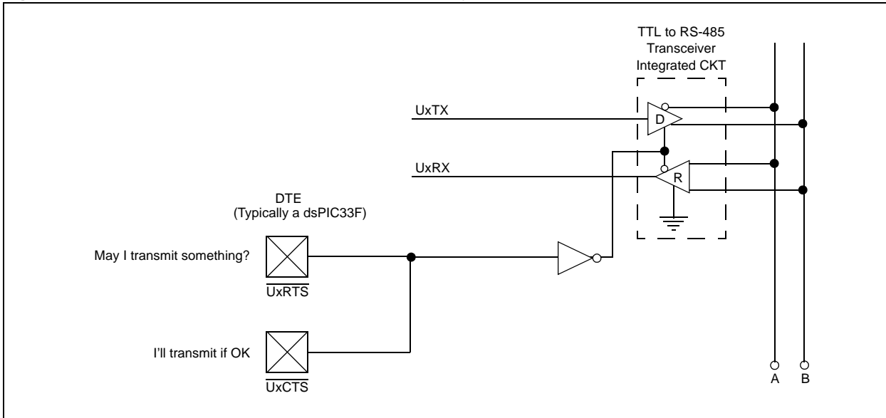
Figure 17-18: \overline{UxRTS}/\overline{UxCTS} Bus Enable for IEEE-485 Systems (RTSMD = 1)
