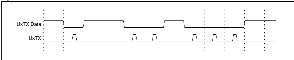
Figure 17-19: IrDA® Encode Scheme
