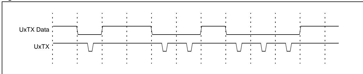
Figure 17-20: IrDA® Encode Scheme for '0' Bit Data
