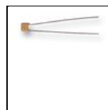
CAP, CERAMIC, 0.1UF, 50V, X7R VISHAY K104K15X7RF53L2
