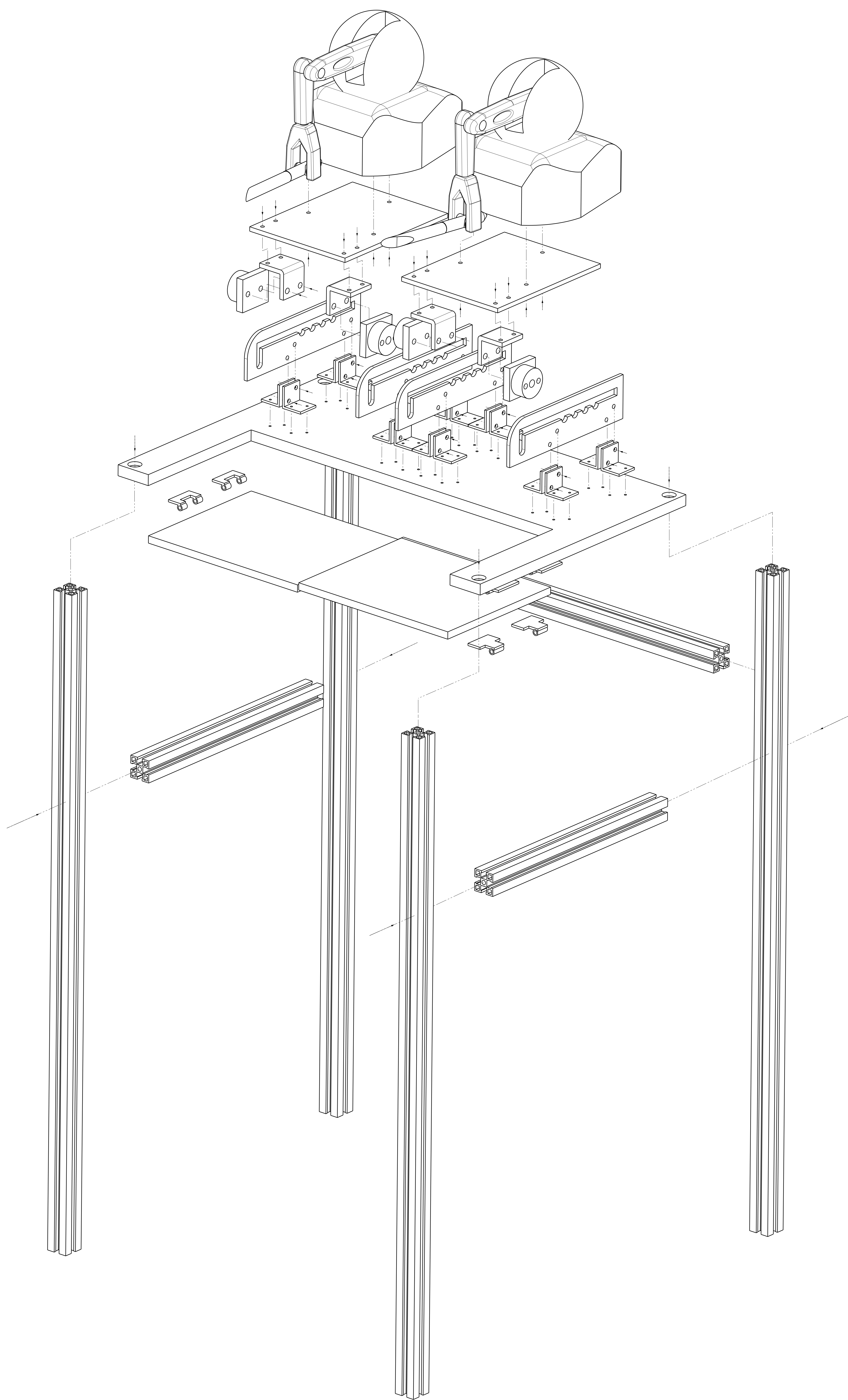
Isometric view Scale: 1:2
