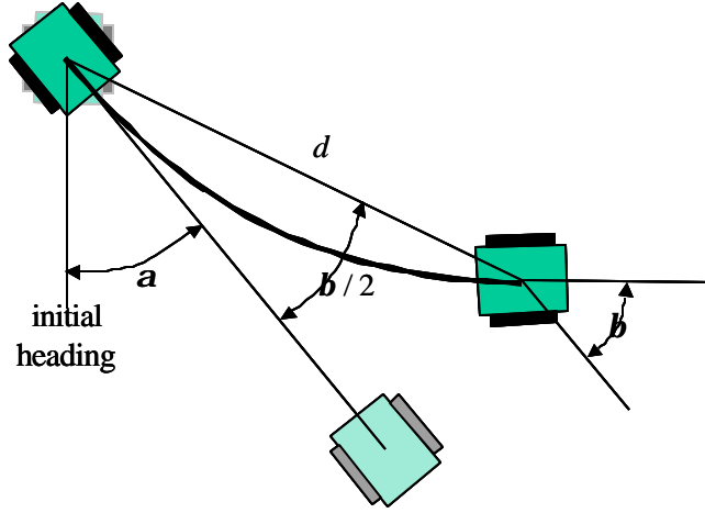
Figure 5: Vector command, (a, d) , with the deviation from straight-line motion.
