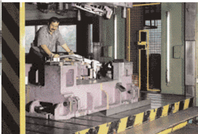
PLS/LSI with two protective fields. One machine can continue to be operated whilst the other is being set up. This results in clear time savings.
