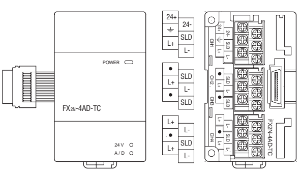
FX2N-4AD-TC
