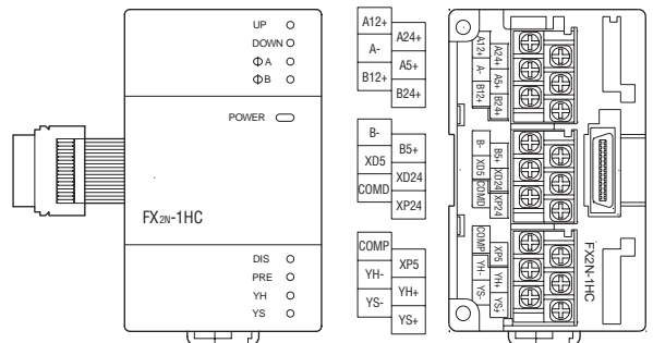
FX2N-1HC
