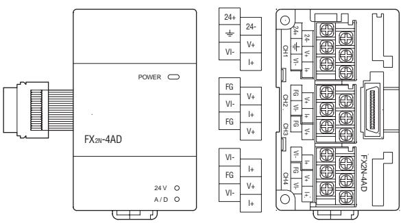
FX2N-4AD
