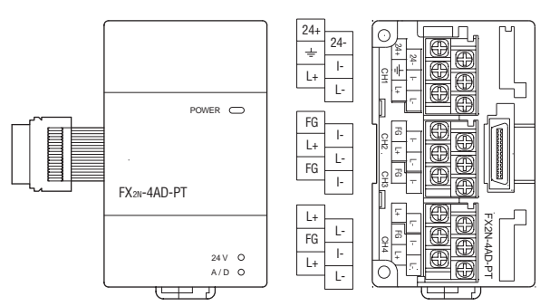
FX2N-4AD-PT
