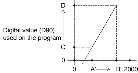
Digital values (D8112 and D8113) practically AD-converted
