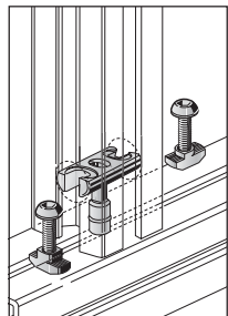
Bolt Connector Kits 3-19 & 3-20
