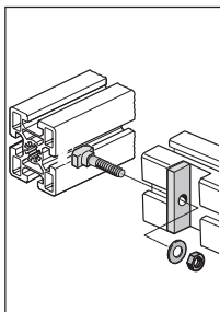
Cross Connector Kit 3-20
