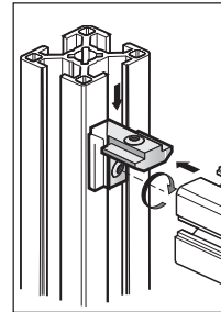
Inside-to-Outside Gussets 3-12
