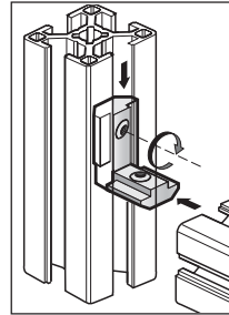
Inside-to-Inside Gussets 3-13
