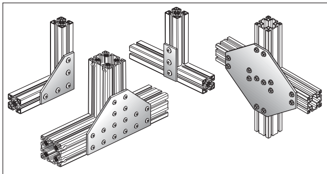
Corner, T-Junction, Rectangular, and Cross Junction Joining Plates 3-33 to 3-36
