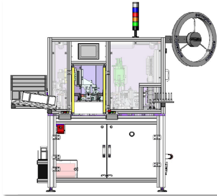
Figura 74 – Vista lateral do “ Secondary spool ASM equipment ”.
