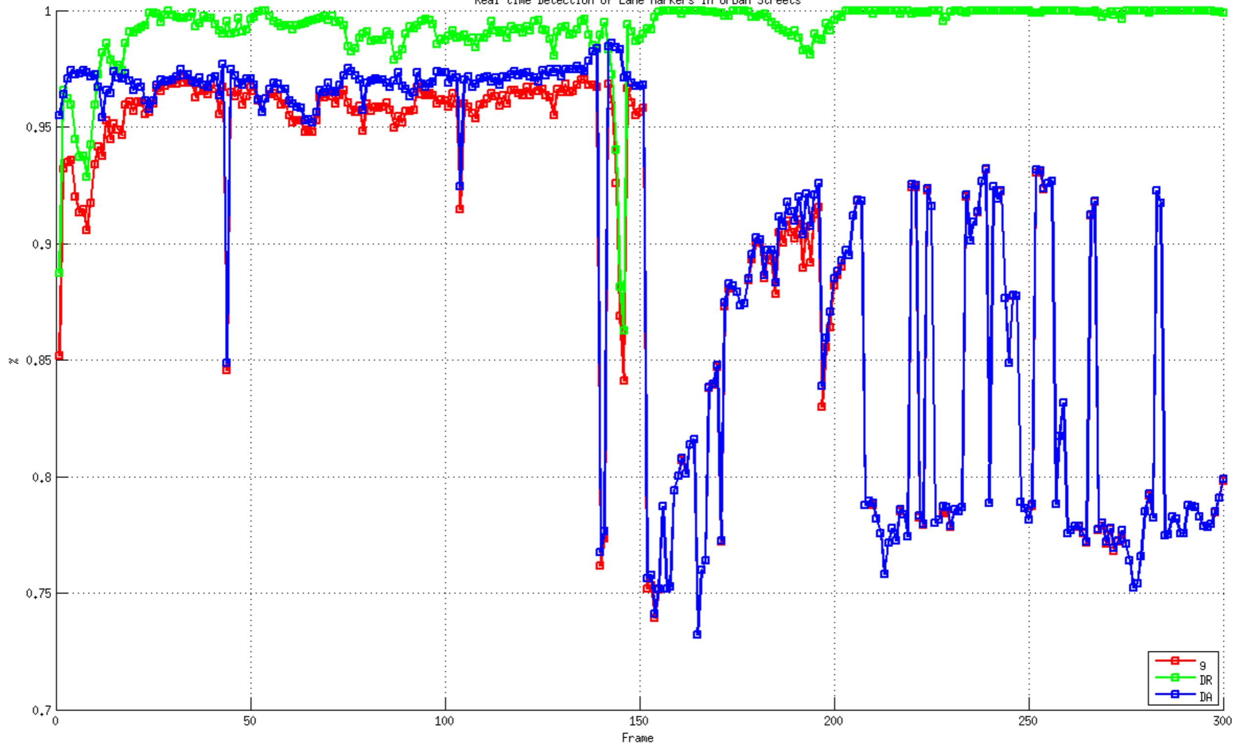
Real time Detection of Lane Markers in Urban Streets
