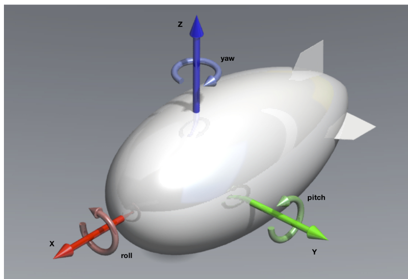
Figure 3.1: Reference axis considered, for future analysis.
