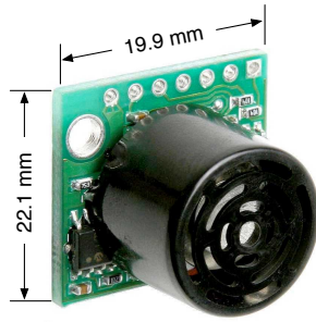
Figure 4.5: Maxbotix Sonar, with the external dimensions.
