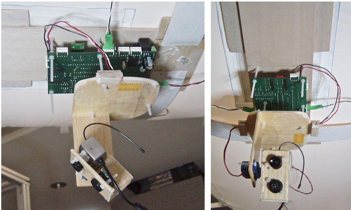
(a) Side view of the assembled control board, camera and sonar. (b) Frontal view of the control system.
