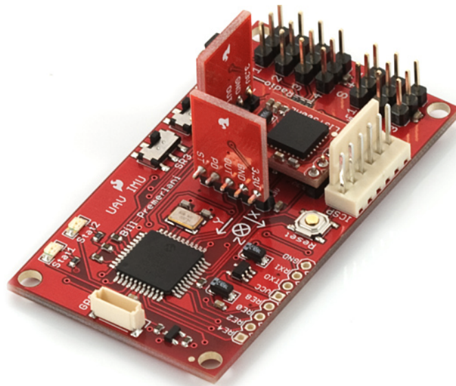
Figure 2.2: The UAV DevBoard, an three-axis autopilot development board developed by Bill Premerlani.
