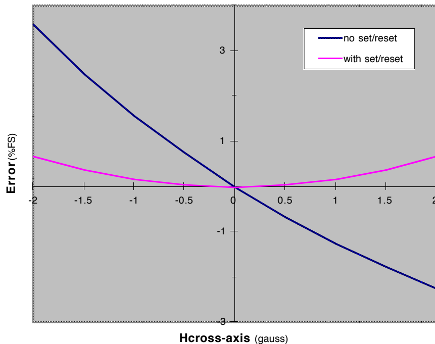
Cross-Axis Field Effect (Hsensitive=0.5 gauss)
