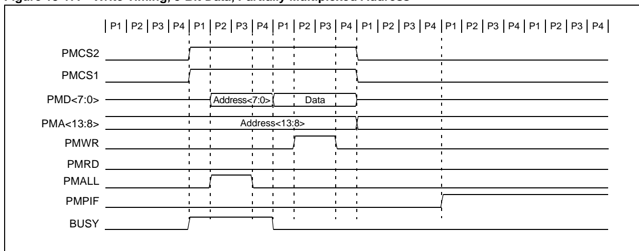
Figure 13-17: Write Timing, 8-Bit Data, Partially Multiplexed Address
