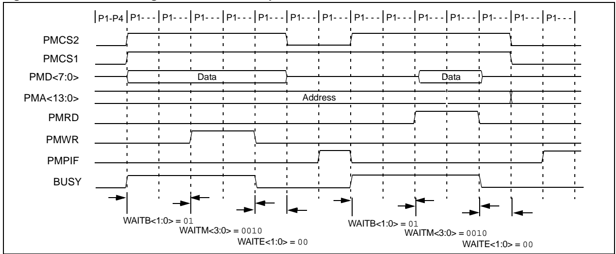
Figure 13-14: Read Timing, 8-Bit Data, Demultiplexed Address, Wait States Enabled
