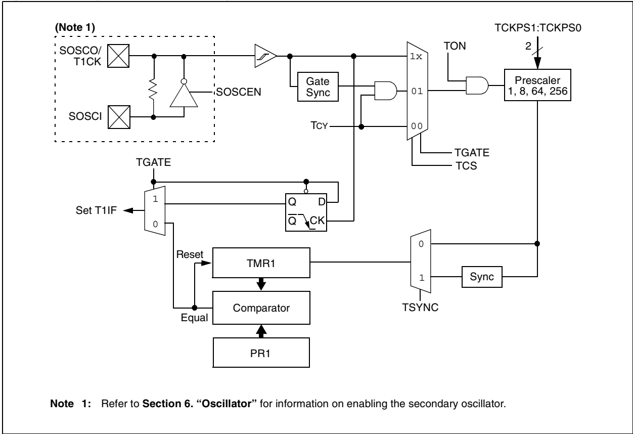
Figure 14-1: Type A Timer Block Diagram
