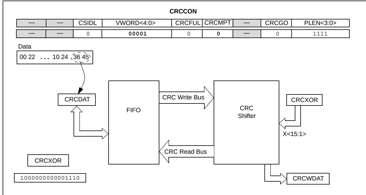
Figure 36-5: Write Data to CRCDAT Register
