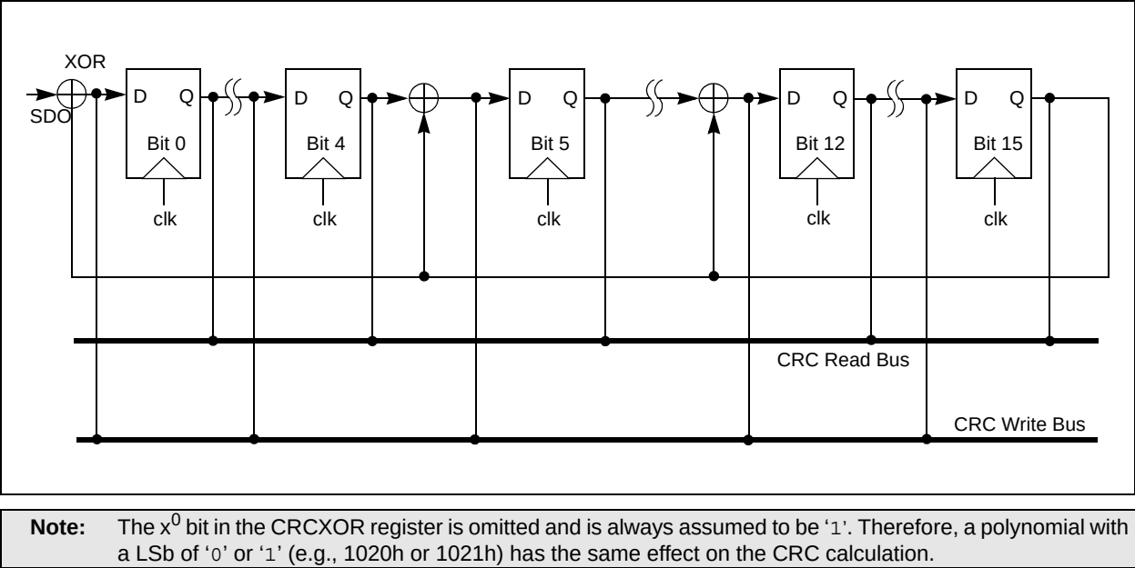
Figure 36-3: CRC Generator Reconfigured for x^{16} + x^{12} + x^5 + 1
