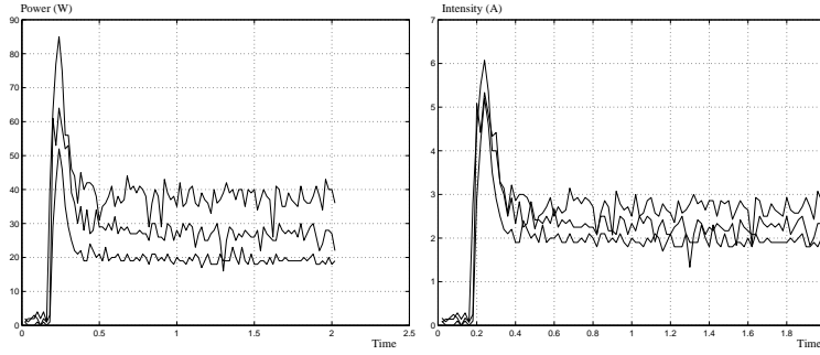
Figure 14: Power and intensity output for various values of the tension
