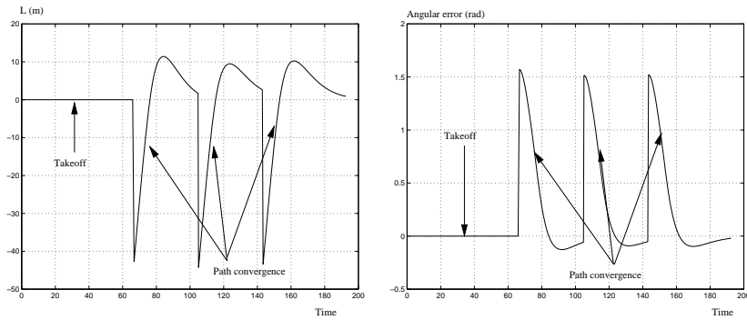
Figure 24: Lateral and angular errors evolution
