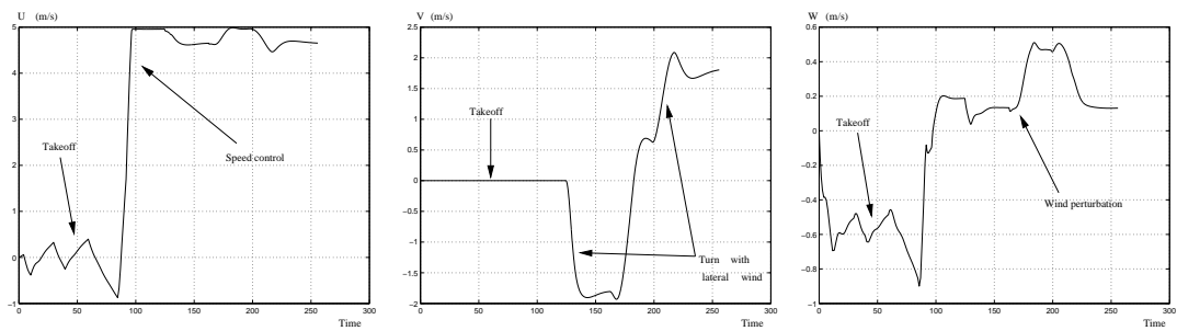
Figure 27: Evolution of the velocity components in the body fixed frame
