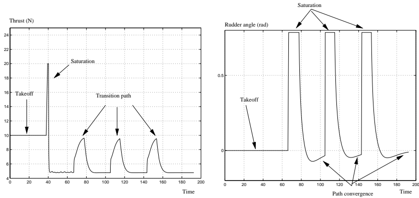
Figure 23: Actuators activity
