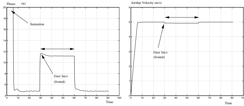
Figure 12: Velocity stabilization with frontal gust
