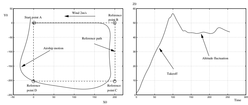
Figure 26: Lateral motion and time evolution of the altitude
