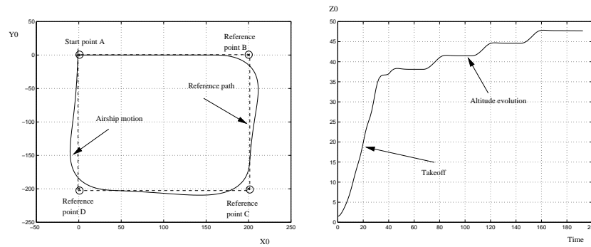
Figure 20: Lateral motion and altitude variation
