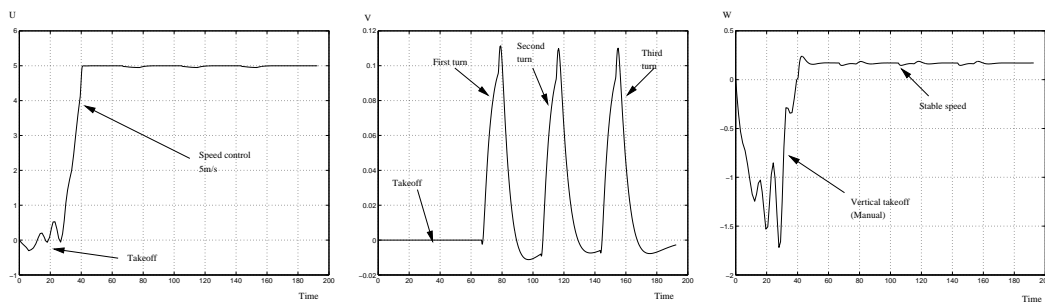
Figure 21: Velocity components with respect to the local frame
