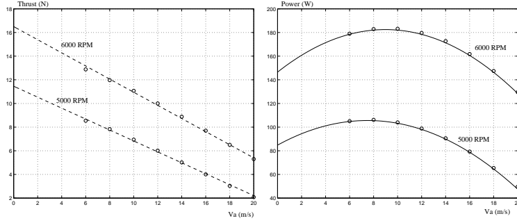
Figure 13: Thrust T and absorbed power P vs aerodynamic velocity V_a for 5000 rpm and 6000 rpm
