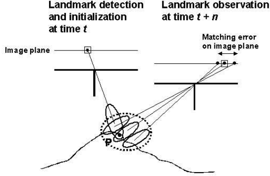
Figure 36: Principle of the combination of the matching and stereovision errors. The points located in the square box are the projection of P on the image plane. Small ellipses indicate stereovision errors, the large dotted ellipsoid is the resulting observation error.
