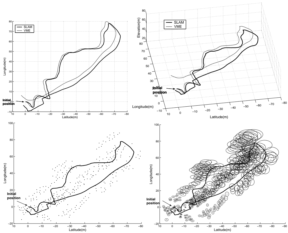
Figure 41: An other result of our SLAM implementation with a sequence of 400 stereovision pair. Top image show the reconstructed trajectory in orthogonal projection and in 3D. Bottom images show the 340 landmarks mapped, with 1\sigma uncertainty ellipses (left: real scale, right: magnified by a factor of 40)
