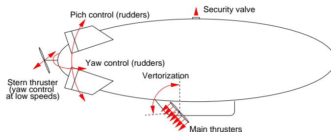
Figure 2: The various control parameters of Karma
