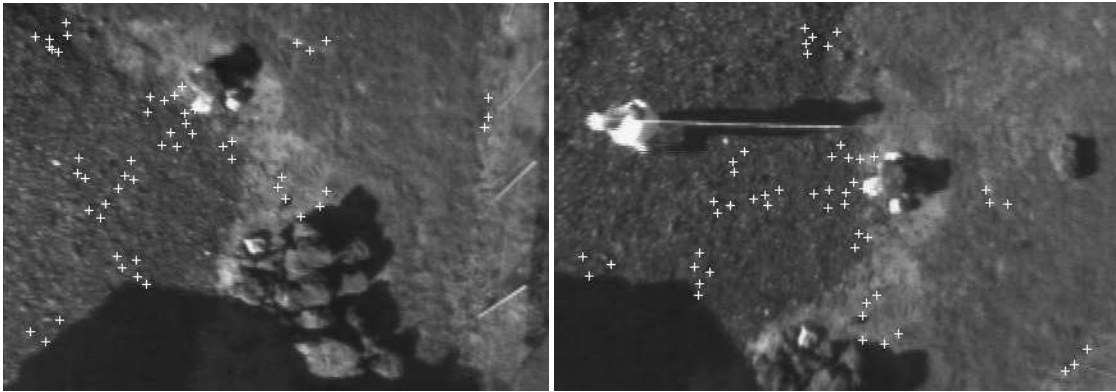
Figure 33: A result of interest point matching between two non-registered aerial images
