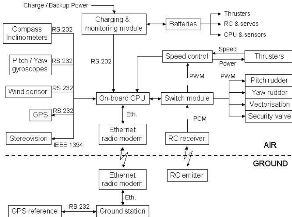
Figure 3: The hardware architecture of Karma, showing the various formats of information exchanges between the instruments. Note that the GPS reference corrections are transmitted via the radio Ethernet link.
