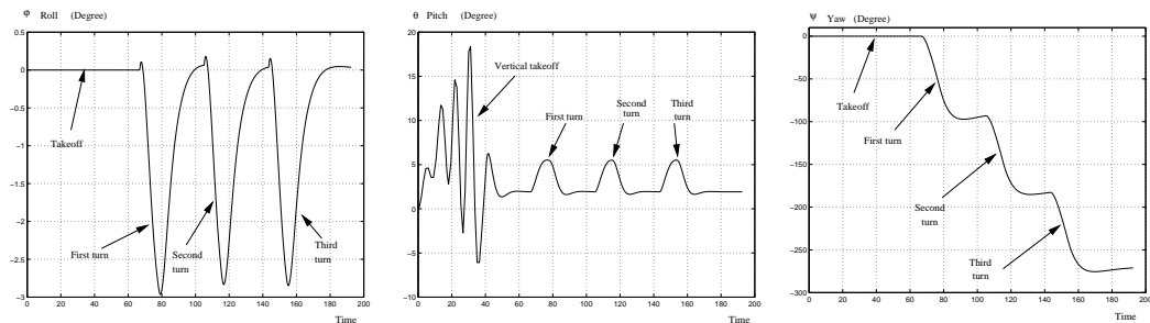
Figure 22: Airship's attitude
