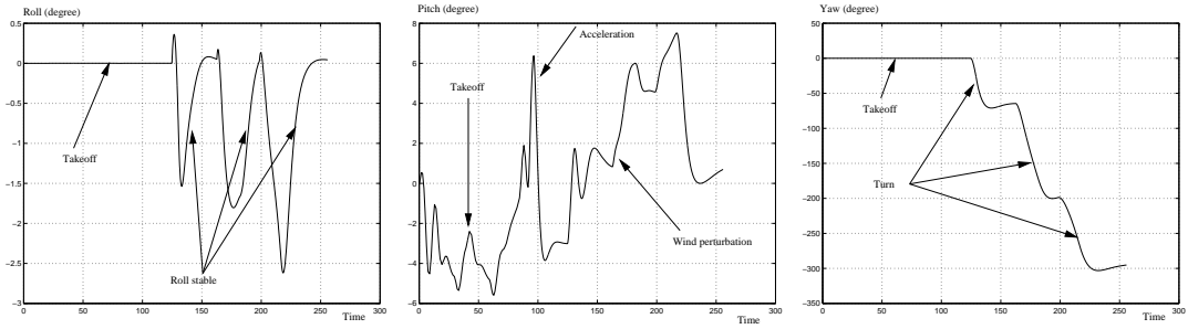
Figure 28: Airship's attitude
