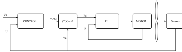
Figure 11: The embedded velocity controller
