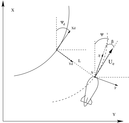
Figure 17: Path following
