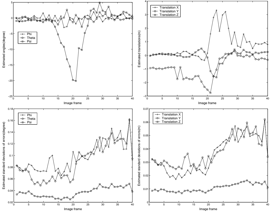
Figure 37: The motion parameters computed by the visual motion estimation algorithm between consecutive frames along a 40 images sequence (top), and corresponding estimated errors (bottom). Note that there are no obvious correlation between the image angular and linear distance and the computed errors.
