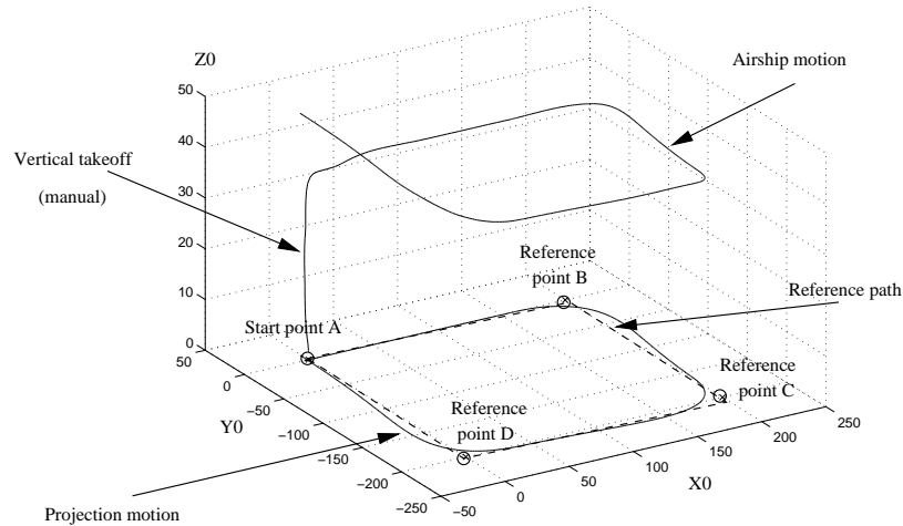
Figure 19: 3D trajectory without wind
