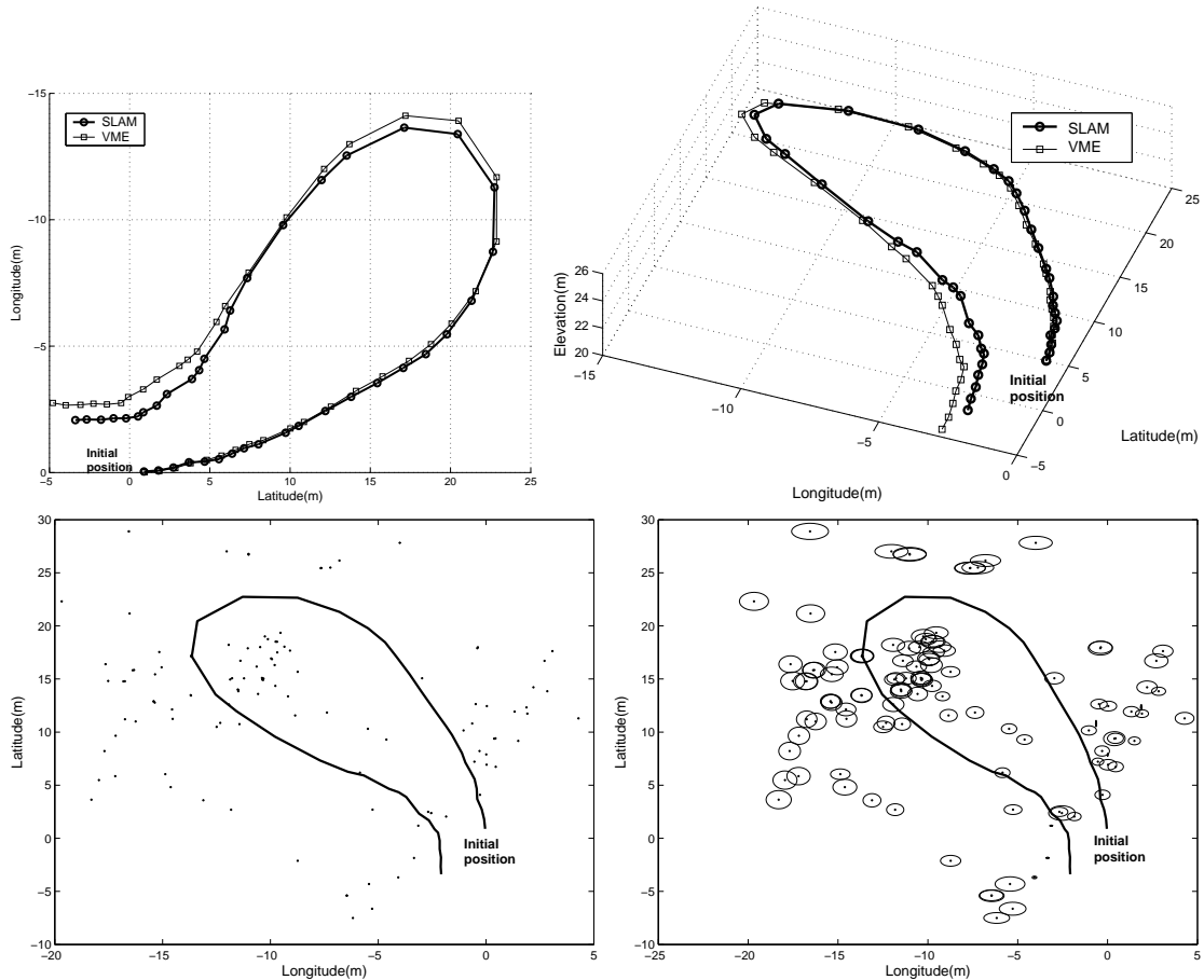
Figure 38: A first result of our SLAM implementation with a sequence of 40 stereovision pair, taken at altitudes ranging from 20 to 25 m. Top image show the reconstructed trajectory in orthogonal projection and in 3D. Bottom images show the 120 landmarks mapped, with 1\sigma uncertainty ellipses (left: real scale, right: magnified by a factor of 40)
