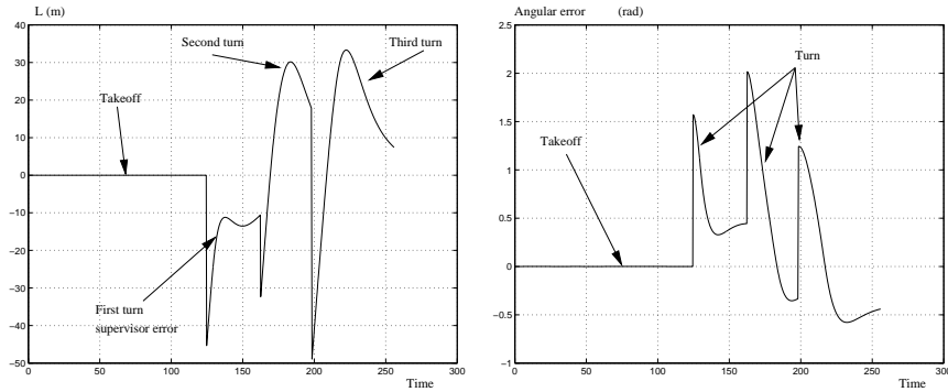
Figure 30: Evolution of position and angular errors
