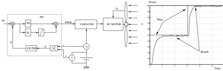
Figure 16: Power control scheme and experiment
