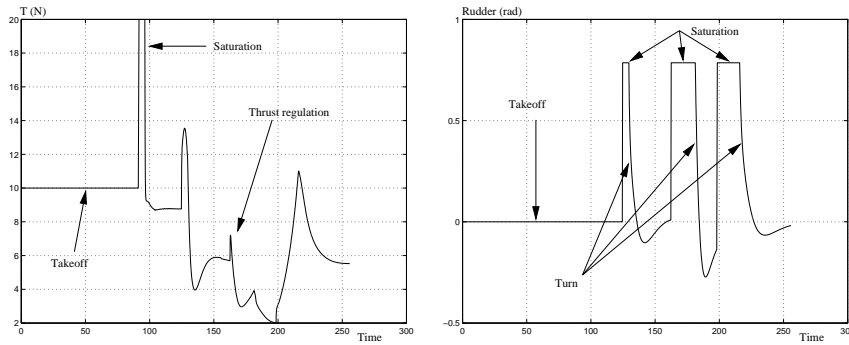
Figure 29: Actuators' activity
