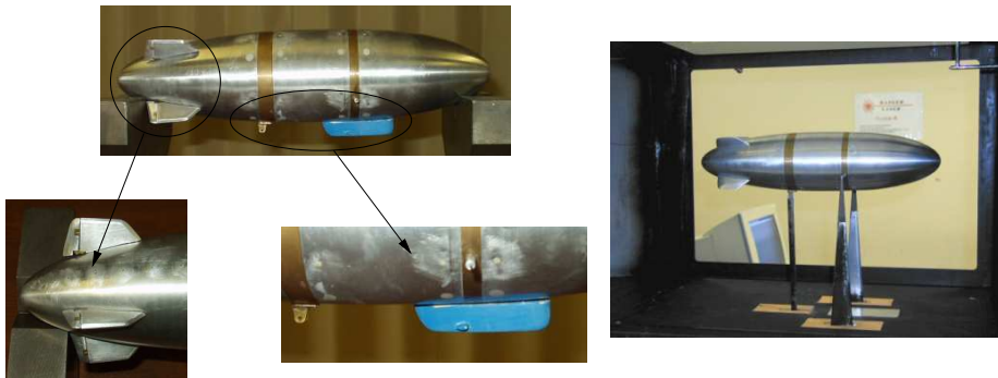
Figure 8: Scale model of Karma in wind-tunnel
