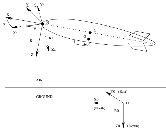
Figure 7: The different frames
