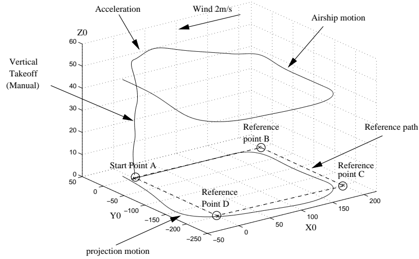
Figure 25: 3D navigation with lateral wind
