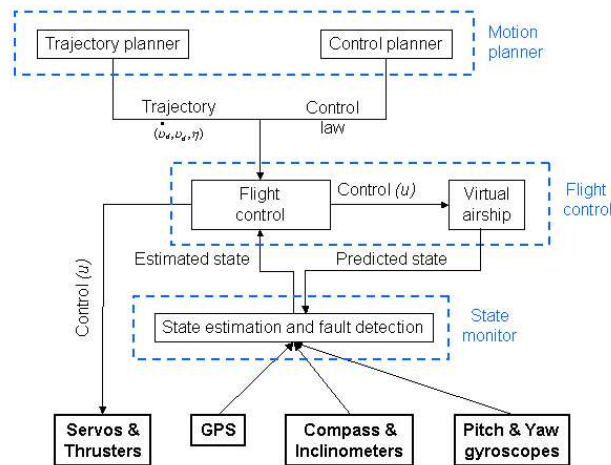
Figure 5: Detailed architecture of the control modules (functional modules of the figure 4 are shown in blue).
