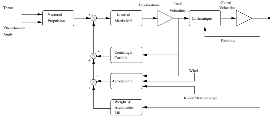
Figure 6: Virtual airship block design
