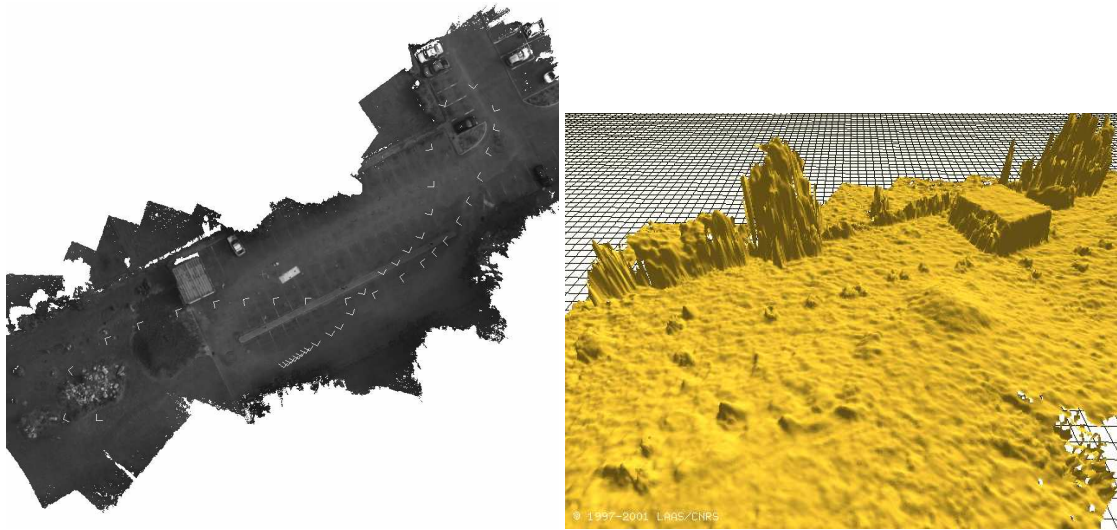
Figure 43: The DEM computed with 100 images, positioned according to the trajectory of figure 40: orthoimage and 3D view of the bottom-left area. The map covers an area of about 3500 m 2 .
