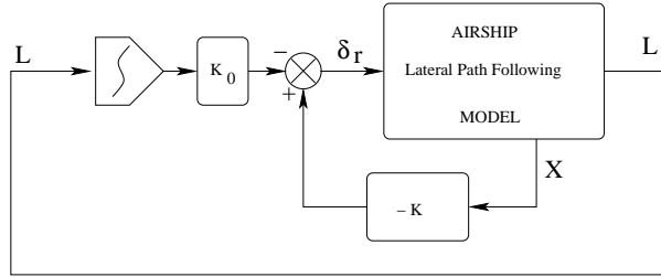
Figure 18: State feedback with integral control
