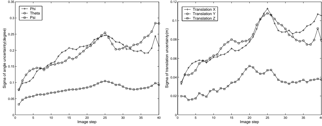
Figure 39: Evolution of the standard deviations of the robot position parameters during the flight shown in figure 38.
