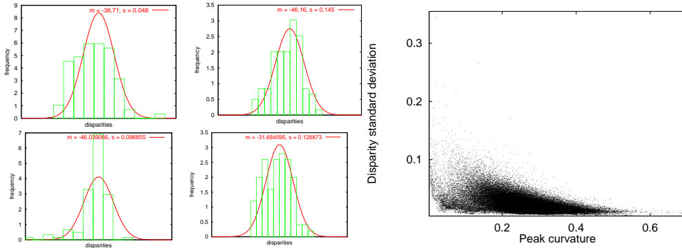
Figure 34: Left: examples of some probability density functions of disparities computed on a set of 100 image pairs, with the corresponding Gaussian fit. Right: Standard deviation of the disparities as a function of the curvature of the similarity score curve at its peak.
