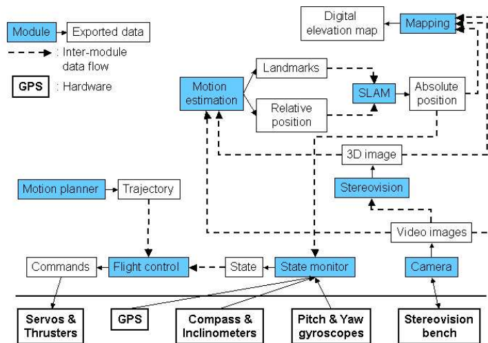
Figure 4: The functional architecture of Karma.
