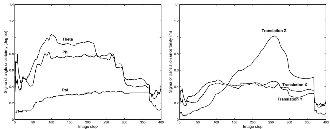
Figure 42: Evolution of the standard deviations of the robot position parameters during the flight shown in figure 41. A drastic decrease of the variances appears in the end, when several landmarks are re-perceived.
