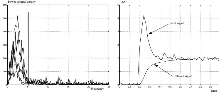
Figure 15: Power spectral density and filtered signal
