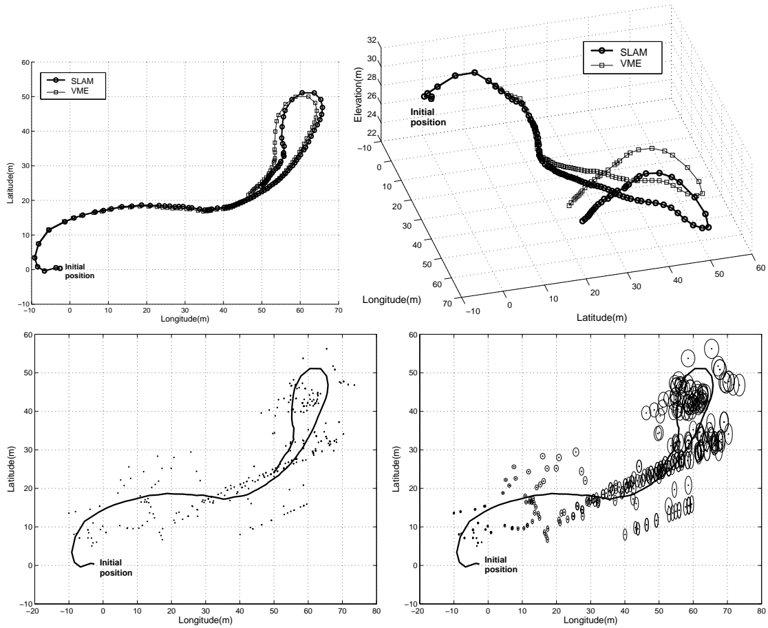
Figure 40: An other trajectory reconstructed with a sequence of 100 images. 320 landmarks have been mapped (the magnification factor of the uncertainty ellipses in the bottom-right image is here 20)
