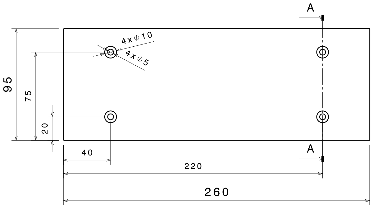
Front view Scale: 1:2
