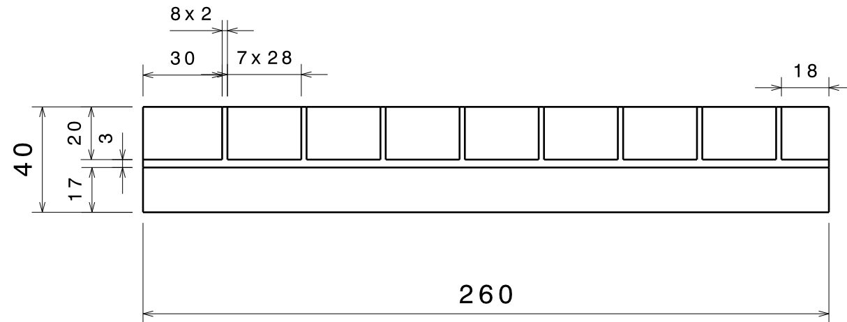
Front view Scale: 1:2
