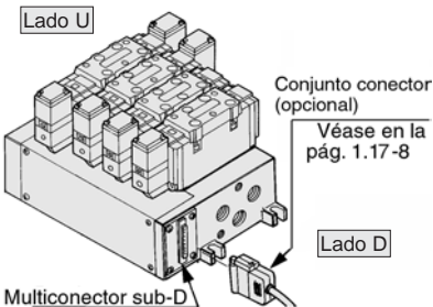
Multiconector sub-D
